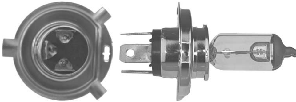
Clear, 12.8 Volt 55/60 Watt Base Type: PX43t-38 Usage: High & Low Beam Halogen Headlight Bulb Industrial Bulb #9003 1 Pc. Per Box
