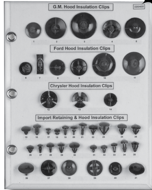
Black Nylon Various Domestic & Import Retaining & Hood Clip Sample Board Sold Each
