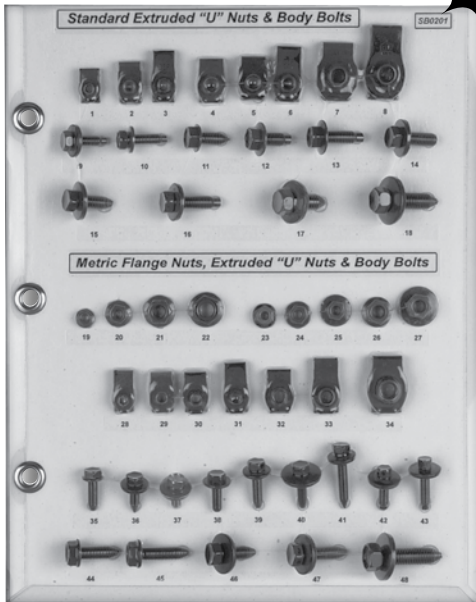
Black & Yellow Zinc Finish Standard Extruded "U" Nuts Hex Flange & Loose Washer Body Bolts Metric Flange Nuts, Extruded "U" Nuts Hex Flange & Loose Washer Body Bolts Sold Each
