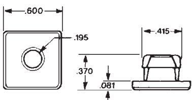
11719 (3907444) Nylon
